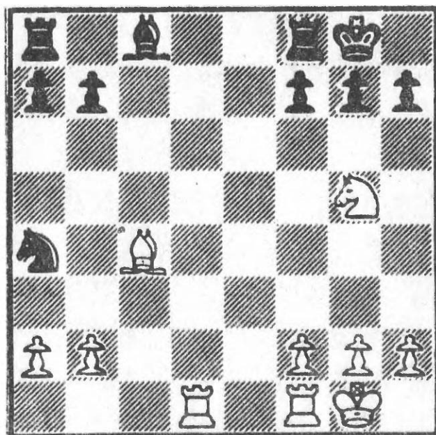
170 After 15...Nxa4
